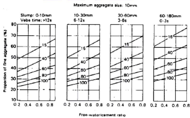
Figure 4a: Recommended proportions of fine aggregate according to percentage passing 600 µm sieve
